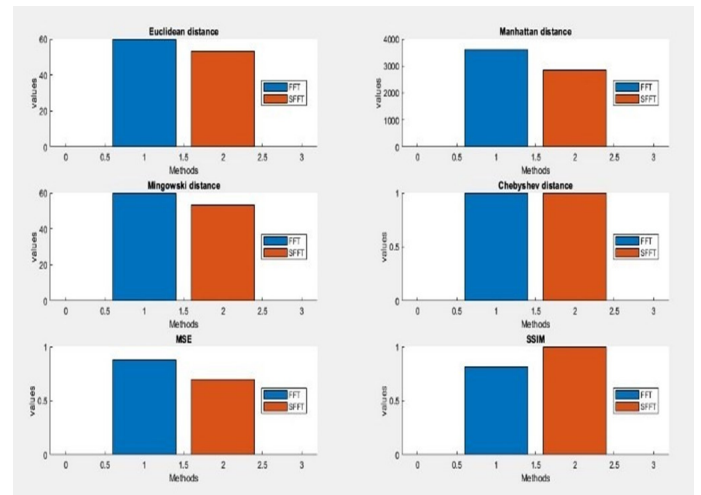
Figure 5. Comparison graphs of FFT and SMART FFT. Note: (■): FFT; (■): SFFT.
